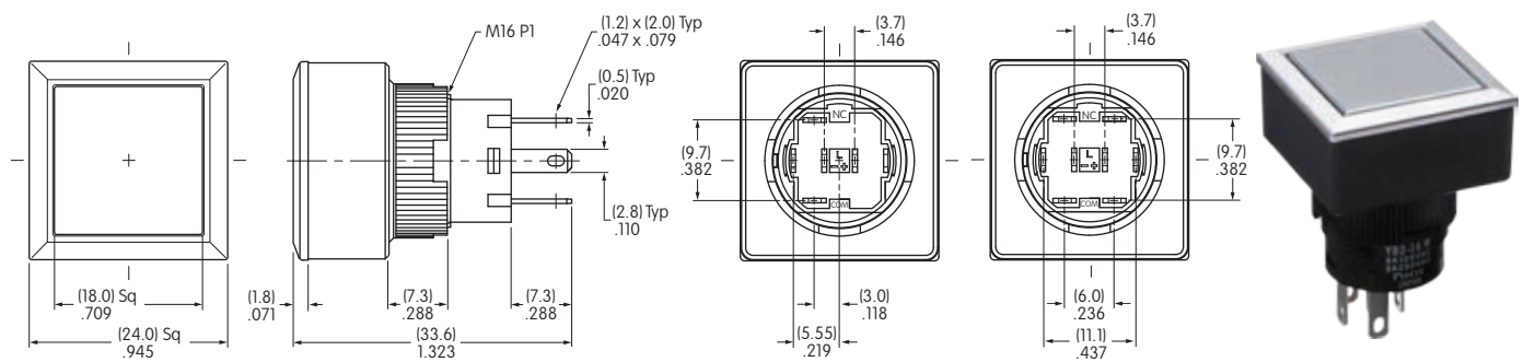
Single Pole
